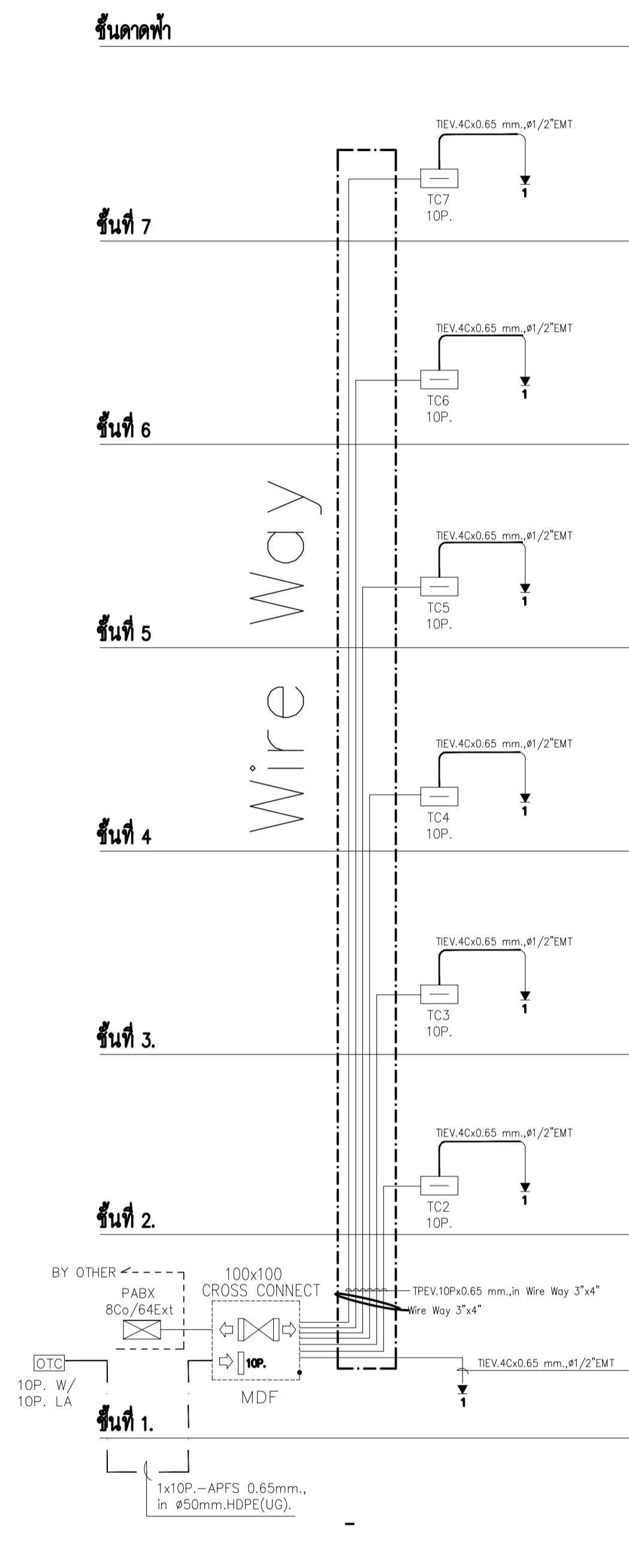
TELEPHONE SYSTEM RISER DIAGRAM
