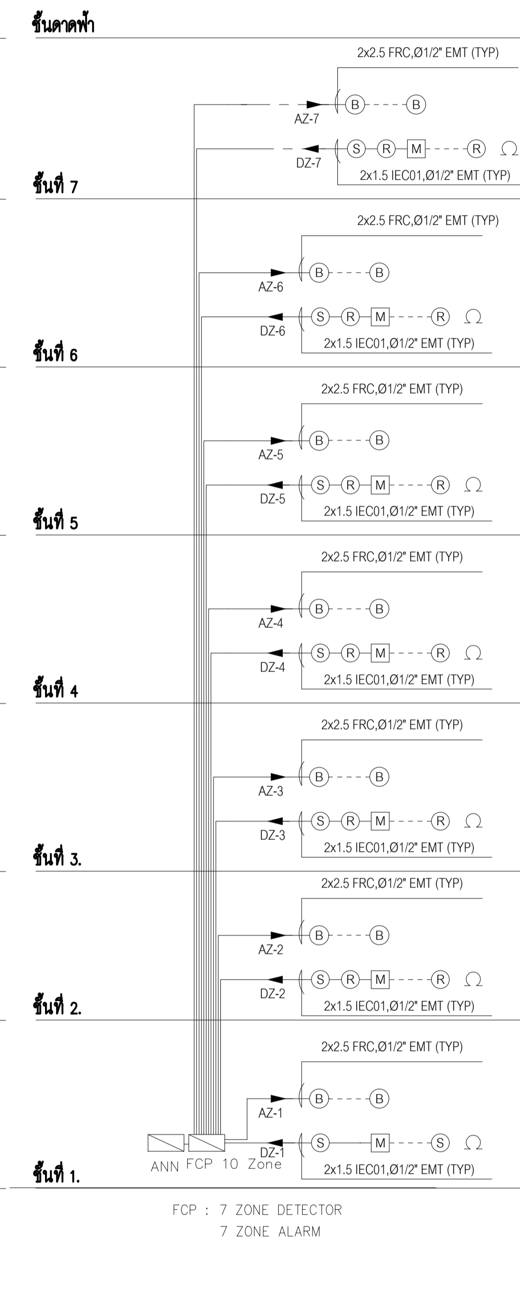
FIRE ALARM SYSTEM RISER DIAGRAM
