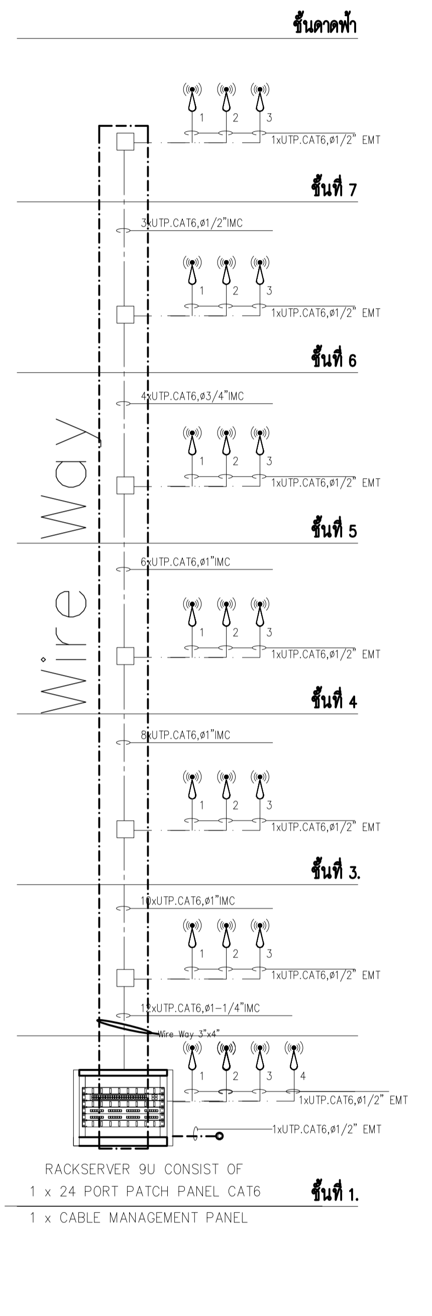
WIFI NETWORK RISER DIAGRAM
