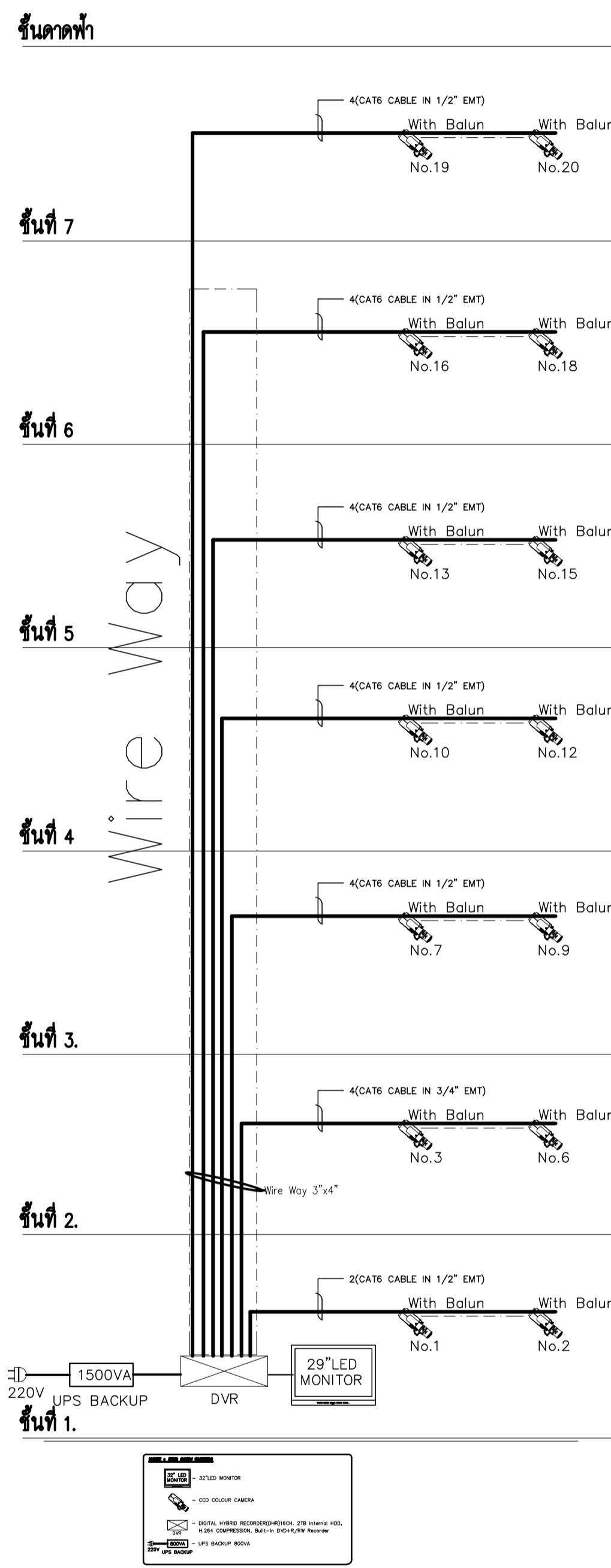
RISER DIAGRAM CCTV SYSTEM
